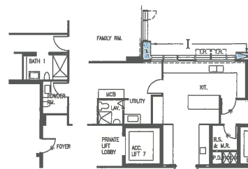
PART PLAN OF KITCHEN, BATH 1 & POWER RM. UNIT C (16/F)
