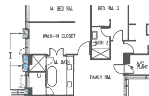
PART PLAN OF M. BATH & M. BED RM. & BATH 3 AT UNIT C (16/F)
