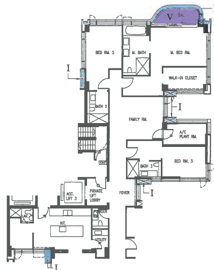
PART PLAN OF BED RM., BATH RM. & KIT. AT UNIT A (16/F)
