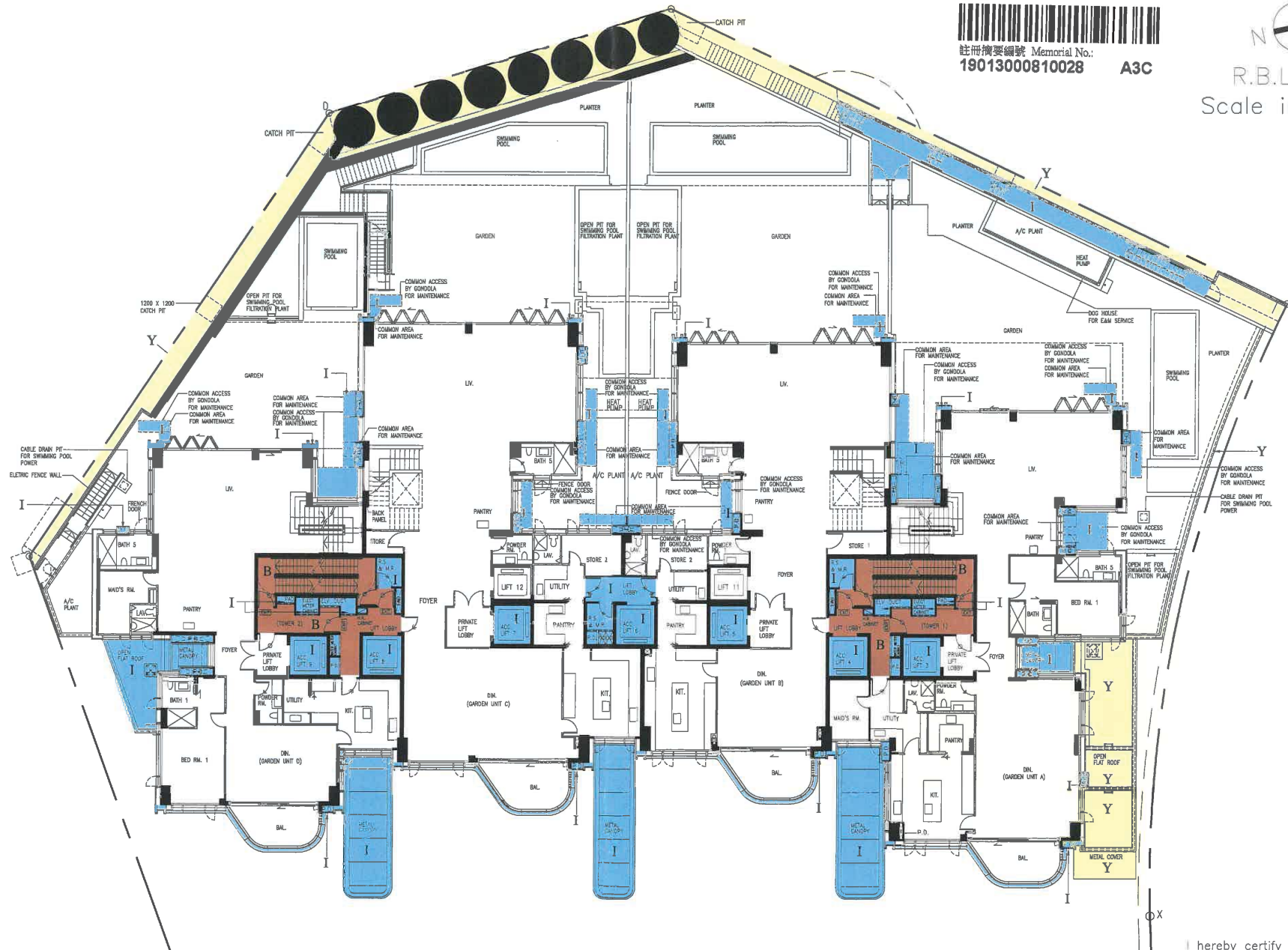
1ST FLOOR PLAN (GARDEN UNIT - LOWER LEVEL)
