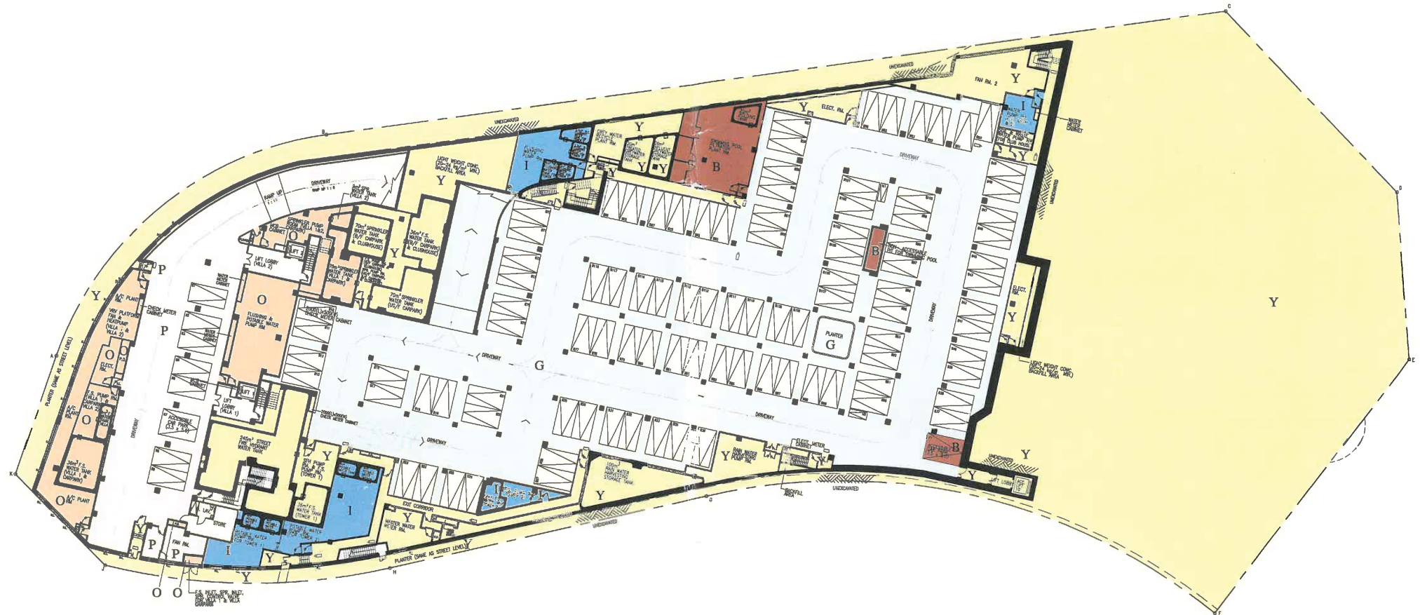
BASEMENT FLOOR PLAN - B/F
